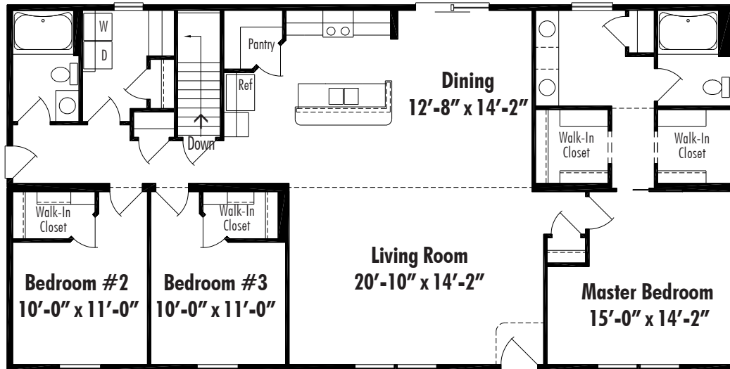
Henderson D Basement 30'x60', 1806 Sq. Ft. Living Area
